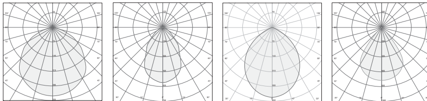
3428 Cierre opal
