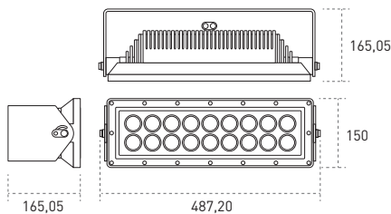
Esdiium Tunnel LED M1 - Horizontal
