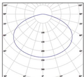
Symmetric optical 150° Optique symmetric 150°
