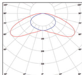
Ref. 3407 Asymmetric optical 150° Optique Asymmetric 150°
