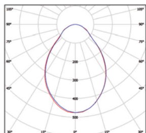
Symmetric optical 80° Optique symmetric 80°
