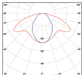
Ref. 3407 Asymmetric optical 80° Optique asymmetric 80°
