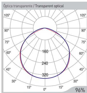
Duris E5 120°
