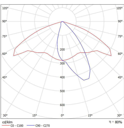
Óp. asimétrica 2 lados 120° log. y 40° trans. a 25° / Asymmetric optic 2 sides 120° Lengthwise and 40°
