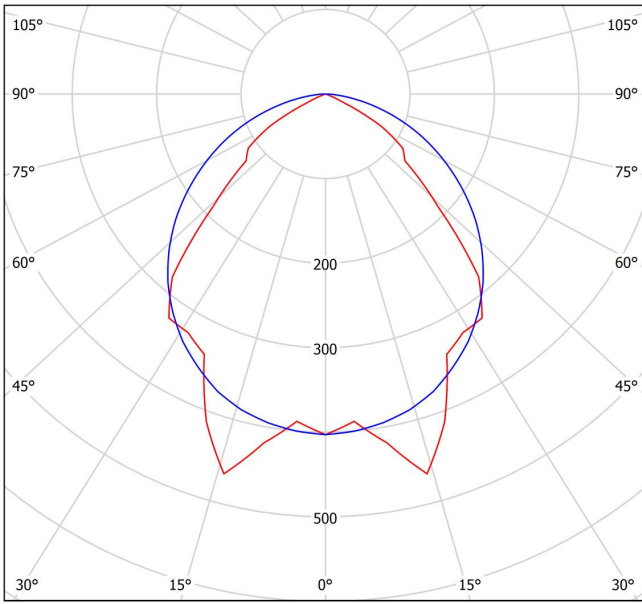
cd/klm \eta = 96\% — C0 - C180 — C90 - C270
